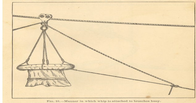
FIG. 10.—Manner in which whip is attached to breeches buoy.
